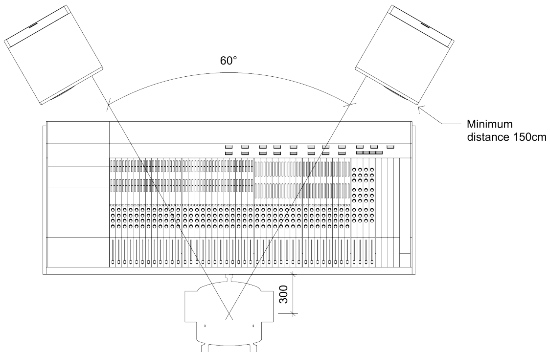
Figure 4b: Typical Stereo M3 MkII layout – top view
