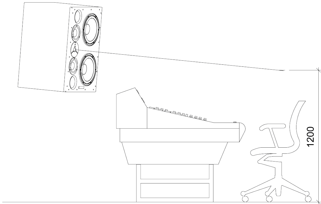
Figure 4a: Typical Stereo M3 MkII layout – side view
