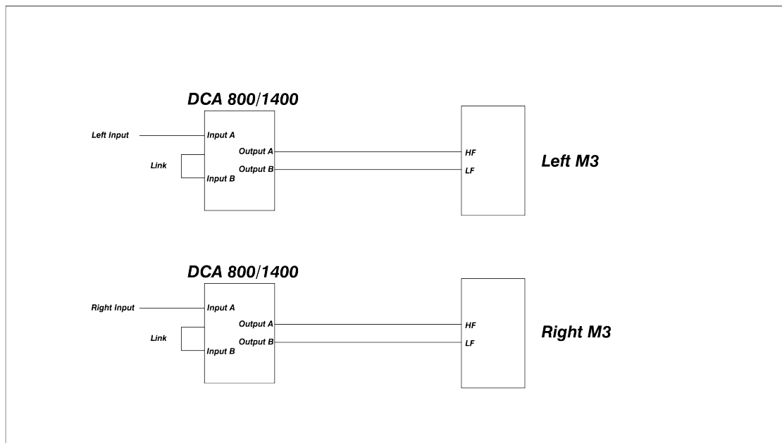
Figure 3: Typical Stereo M3 MkII system with DCA amplifiers (with filters)
