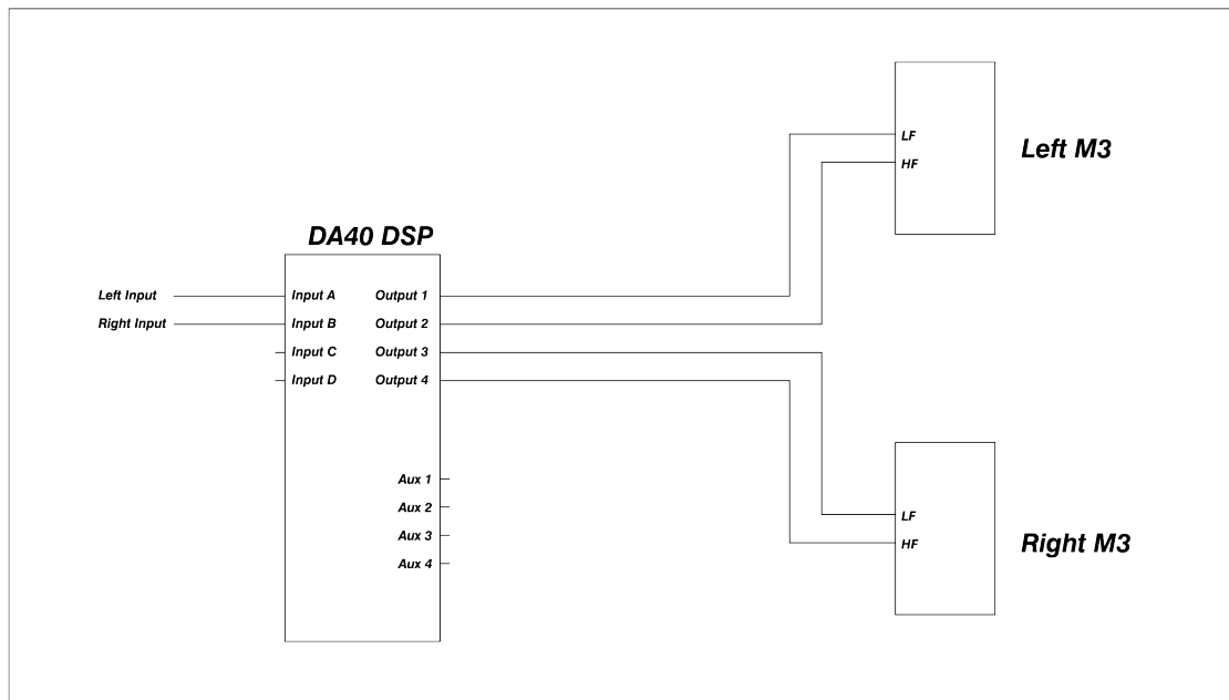
Figure 2: Typical Stereo M3 MkII system with DA40-DSP amplifier
